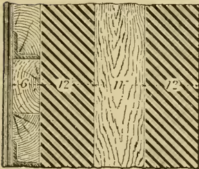
'Inflexible' (England) 1876 Belt & Citadel Armor. Iron Sandwiched
